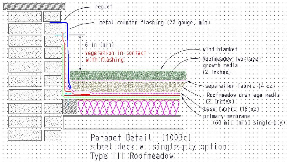
Figure 7. Parapet detail courtesy of Roofscapes, Inc. (TO BE EDITED ASAP)
