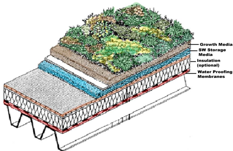
Figure 6. Cross-section diagram showing layers in vegetated roof system (Roofscapes, Inc.)
