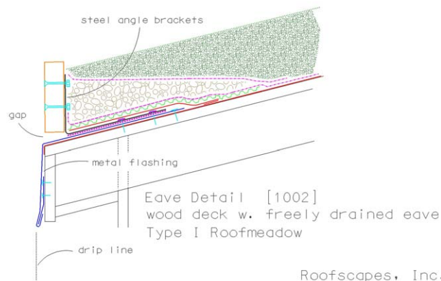
Figure 6. Cross section showing edge detail courtesy of Roofscapes, Inc. (TO BE EDITED ASAP)
